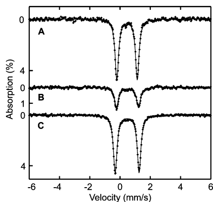
Figure 4. Zero-field Mössbauer spectrum of 8 (A), 7 (B), and 6 (C), acquired at 90 K [experimental data ( \blacklozenge ) and calculated fits (—)].
