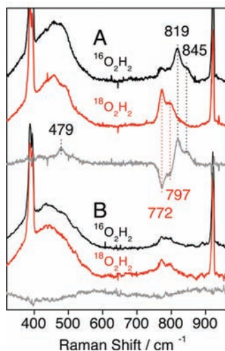
Figure 8. RR spectra of intermediate 6a (A) and its decomposition product (B) obtained with 568-nm excitation at 110 K. Sharp Raman bands below 400 and above 900 \text{cm}^{-1} correspond to solvent vibrations.
