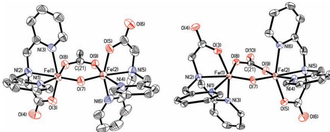
Figure 2. ORTEP diagram of 7 (left) and 8 (right) displaying thermal ellipsoids (50%). For clarity, the diethynylveratrole backbones, the \text{Ar}^{\text{tPrO}} group, and the \text{ClO}_4^- anion are not shown.
