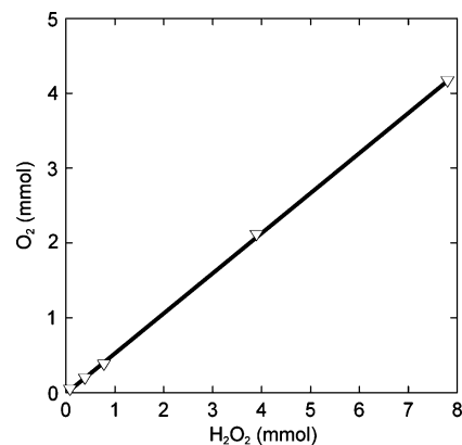
Figure 11. O 2 formation from 0.078 to 7.8 mmol of H 2 O 2 at 0 °C catalyzed by 8 (2 mL of 0.4 mM solution in CH 3 CN/H 2 O, 2:1) and 10 μL of NEt 3 .
