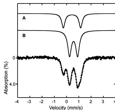
Figure 7. Zero-field Mössbauer spectrum [experimental data ( \blacklozenge )] recorded at 90 K for a frozen solution sample of the product of the reaction of 6 with excess \text{H}_2\text{O}_2 and a trace of \text{NEt}_3 . The sample contained 66% of 6a (B) and 34% of a diiron(III) species (A; \delta = 0.45 \text{ mm/s} and \Delta E_Q = 1.41 \text{ mm/s} ) with Mössbauer parameters similar to those of the starting material.
