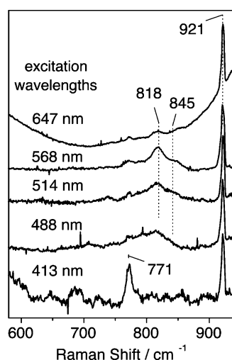
Figure 9. RR spectra of intermediate 6a obtained with different laser excitations at 110 K. All traces are normalized to the 921 \text{cm}^{-1} solvent band.
